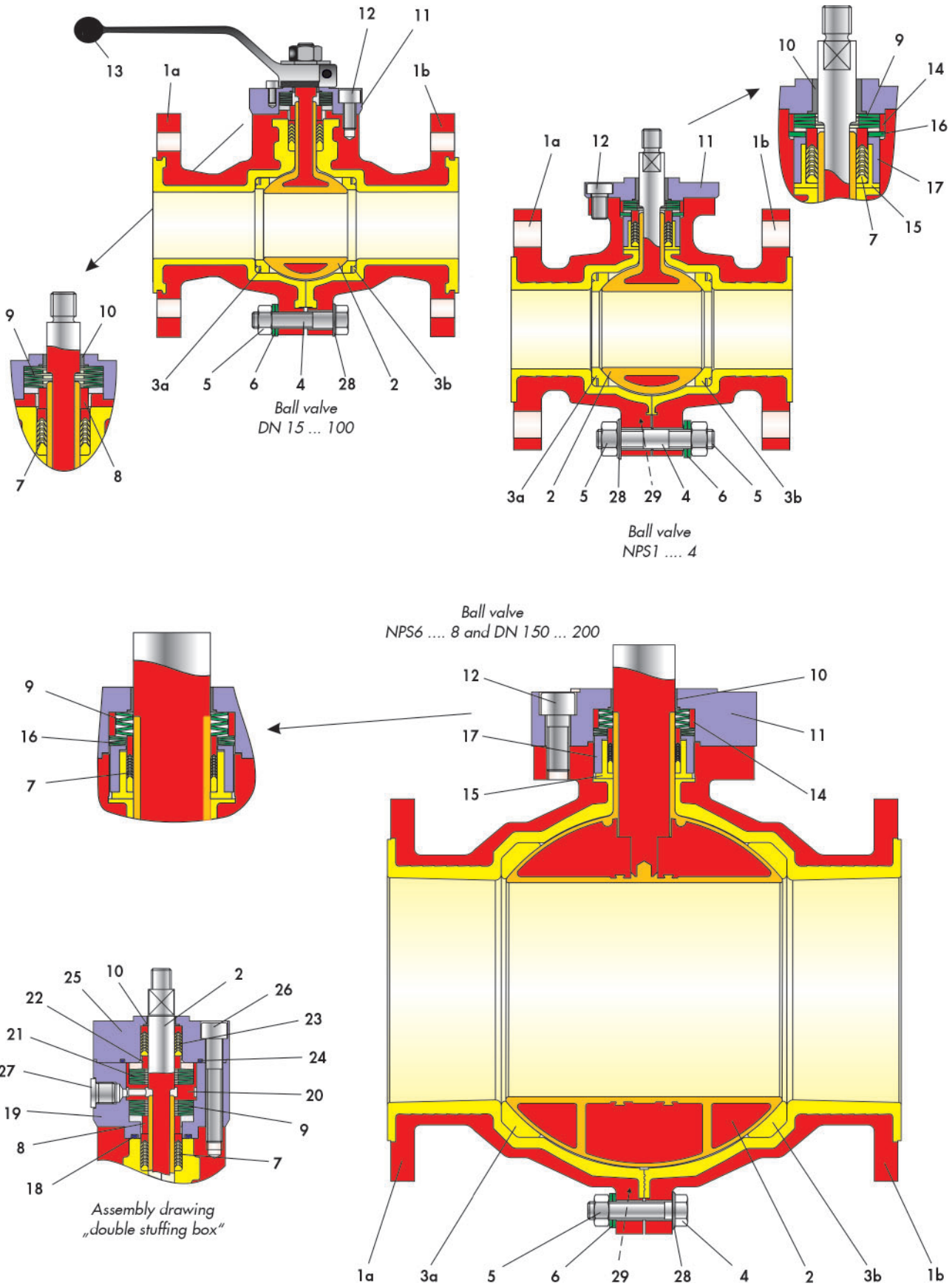
Fig. 3: Sectional drawing of the BR 20a Ball valve
