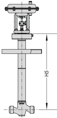
Globe valve with stainless steel body
