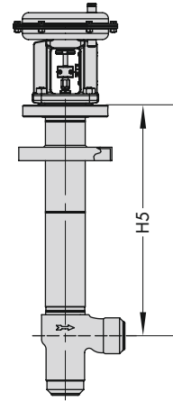
Angle valve with stainless steel body
