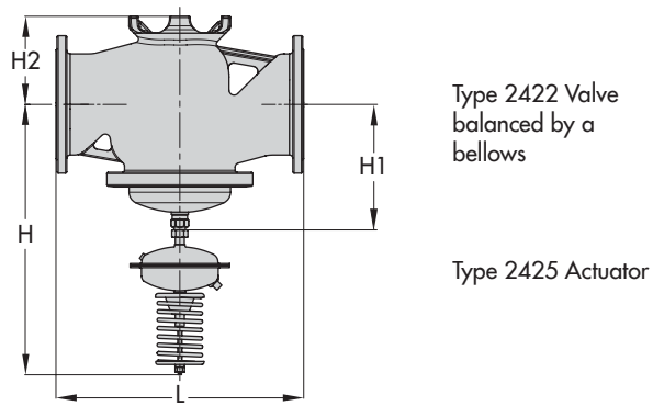
Fig. 4: Dimensional drawing of Type 2422 Valve balanced by a diaphragm with Type 2425 Actuator
