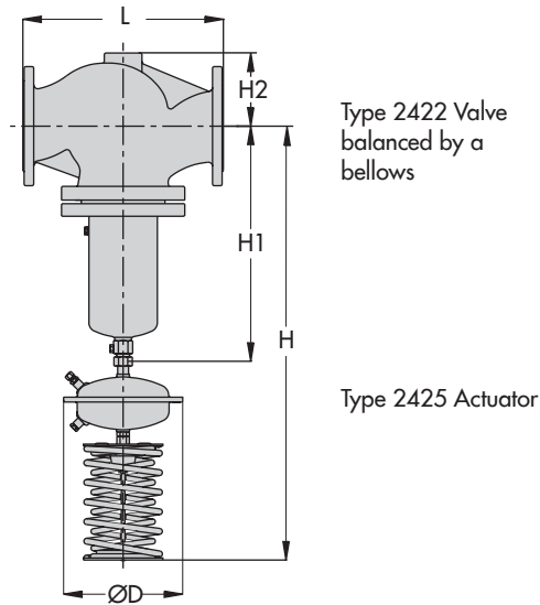
Fig. 3: Dimensional drawing of Type 2422 Valve balanced by a bellows with Type 2425 Actuator
